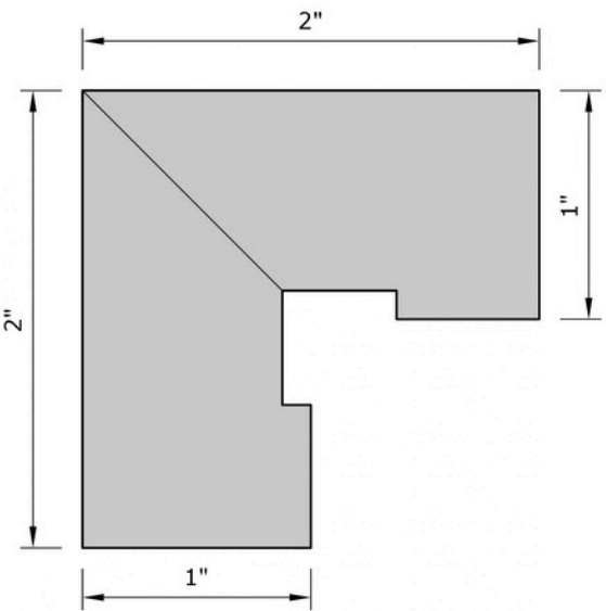
Solid Wood Mitered Outside Corner (panels butt into corner piece)
