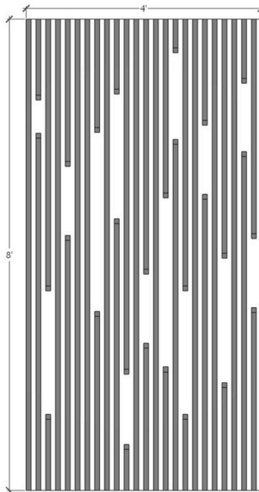
Elevation View
